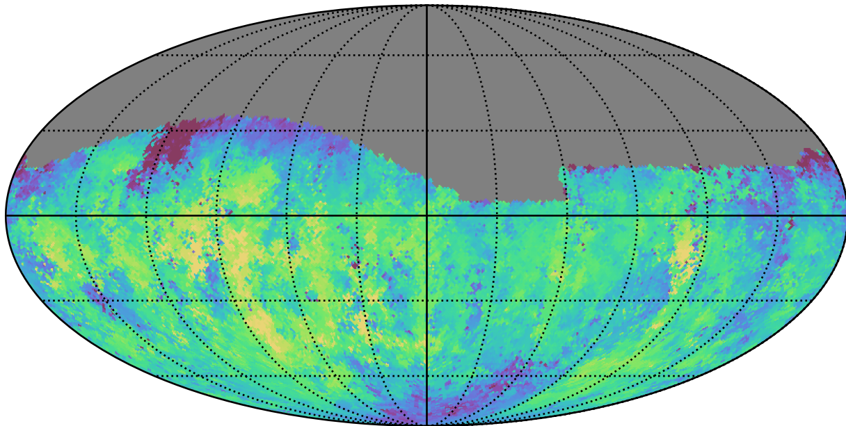
all_long_v3.4_10yrs Yr 1 g band: Median fiveSigmaDepth
