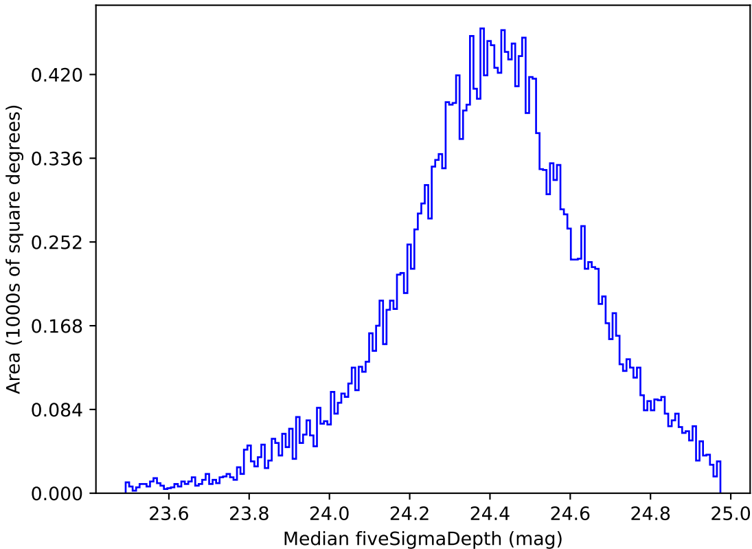
all_long_v3.4_10yrs Yr 1 g band: Median fiveSigmaDepth
