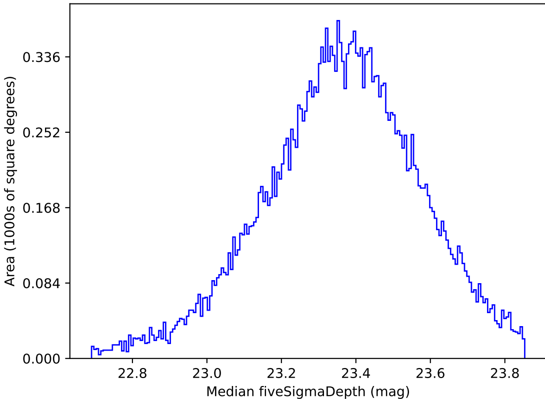
all_long_v3.4_10yrs Yr 1 all bands: Median fiveSigmaDepth
