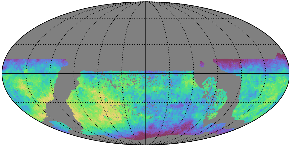
all_long_v3.4_10yrs WFD z band: Median fiveSigmaDepth
