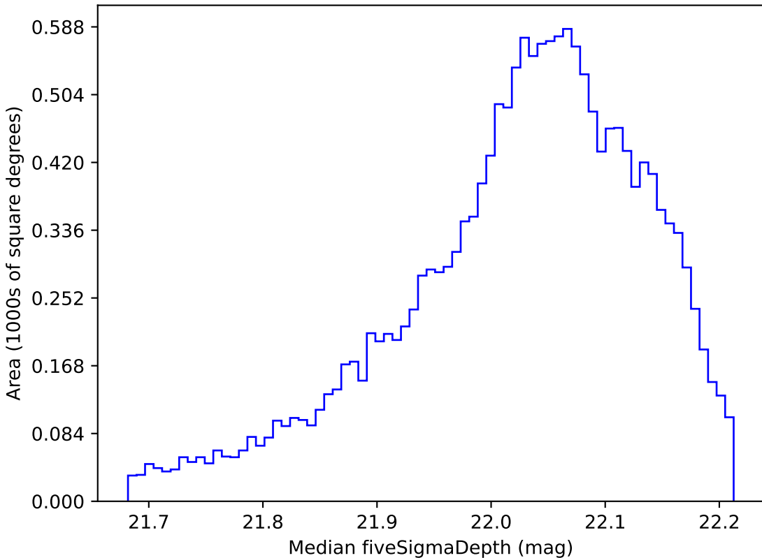
all_long_v3.4_10yrs WFD y band: Median fiveSigmaDepth
