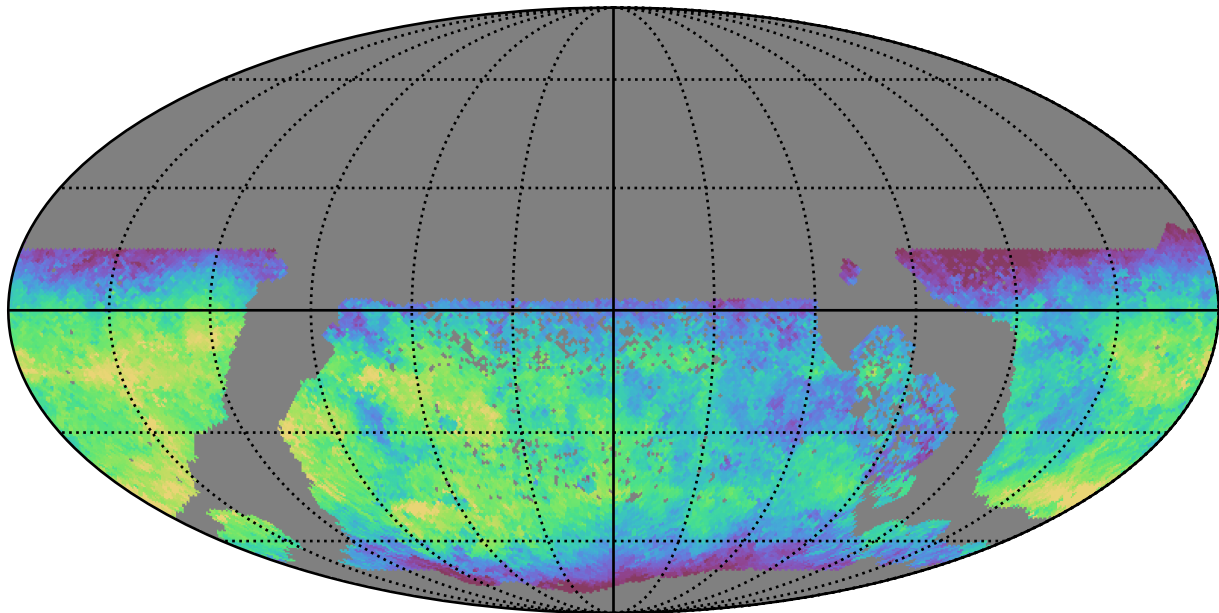
all_long_v3.4_10yrs WFD u band: Median fiveSigmaDepth
