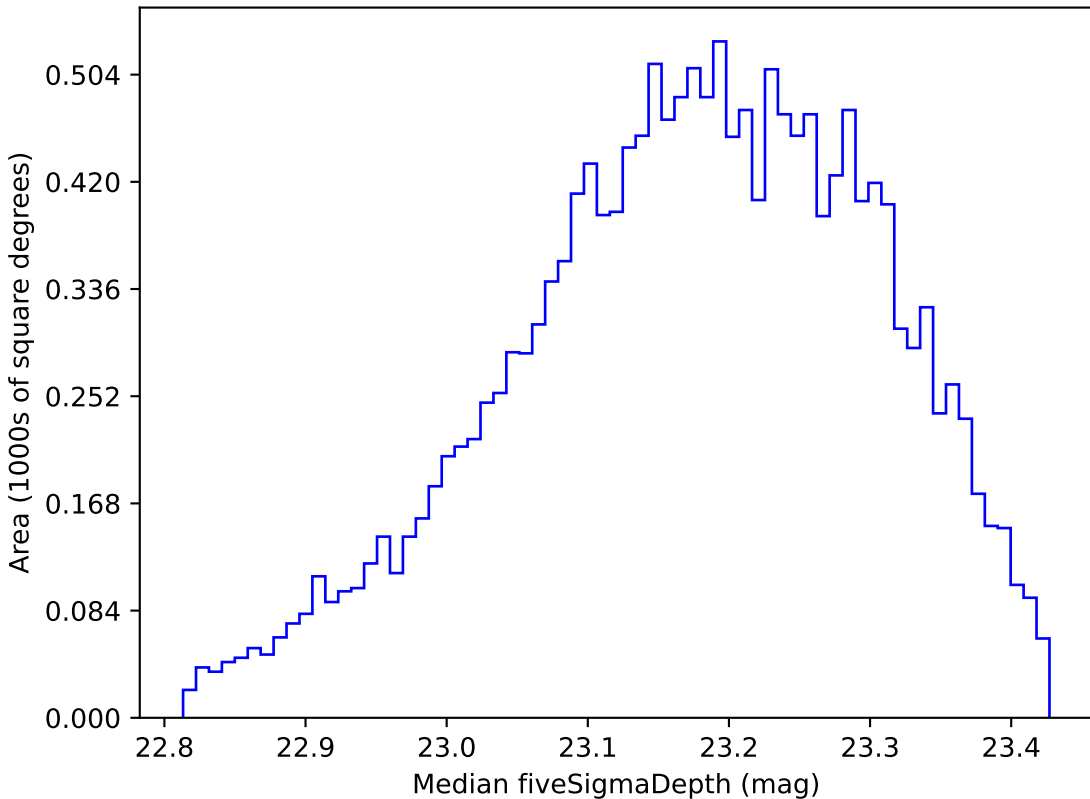
all_long_v3.4_10yrs WFD u band: Median fiveSigmaDepth
