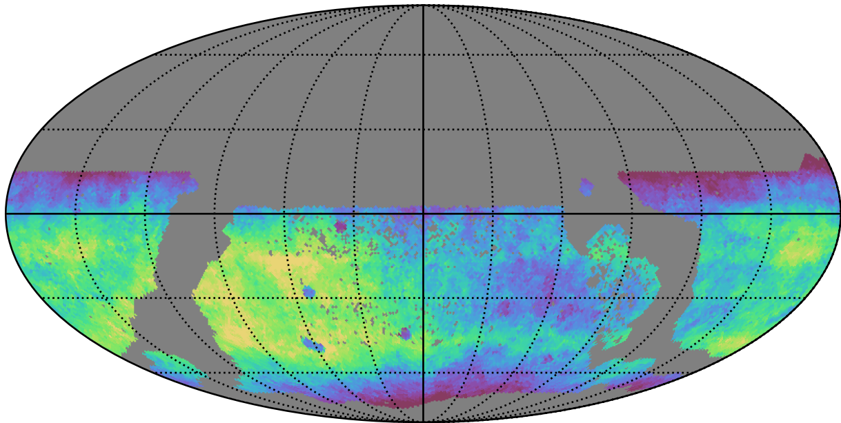
all_long_v3.4_10yrs WFD r band: Median fiveSigmaDepth
