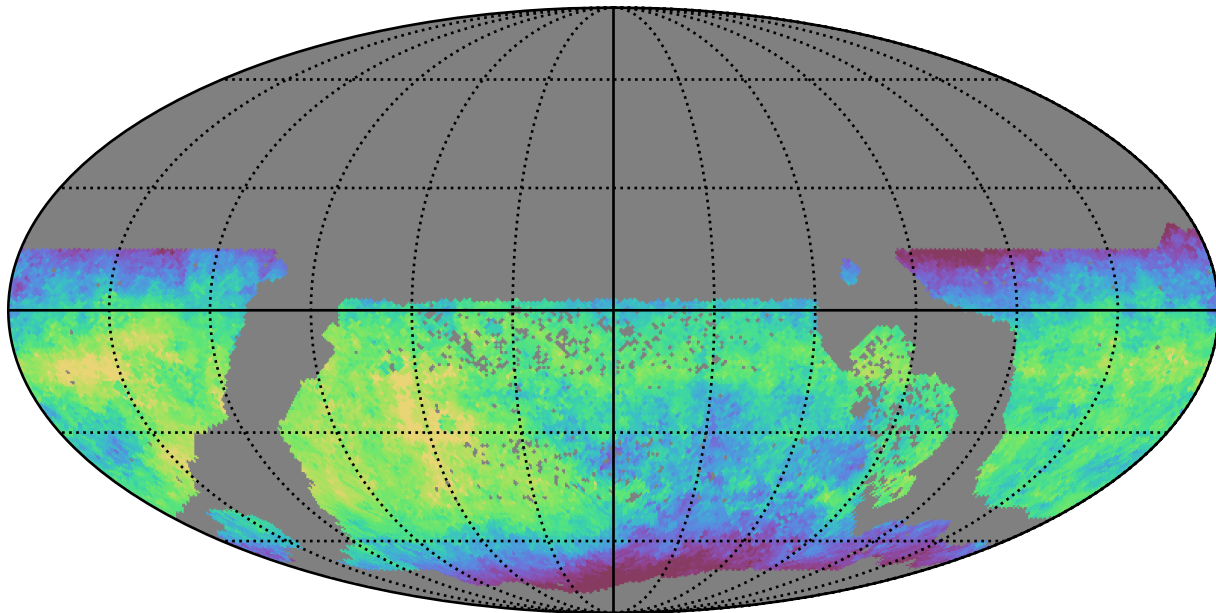
all_long_v3.4_10yrs WFD i band: Median fiveSigmaDepth
