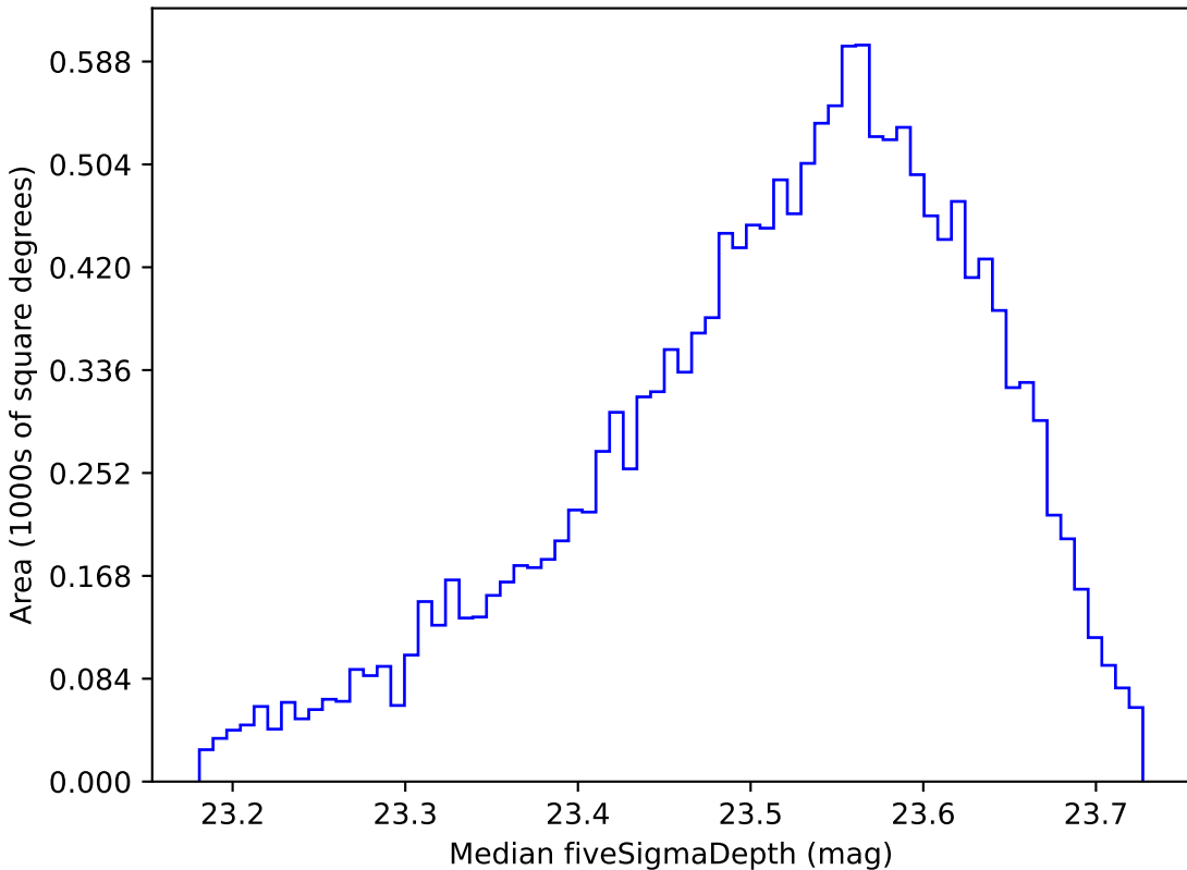
all_long_v3.4_10yrs WFD i band: Median fiveSigmaDepth
