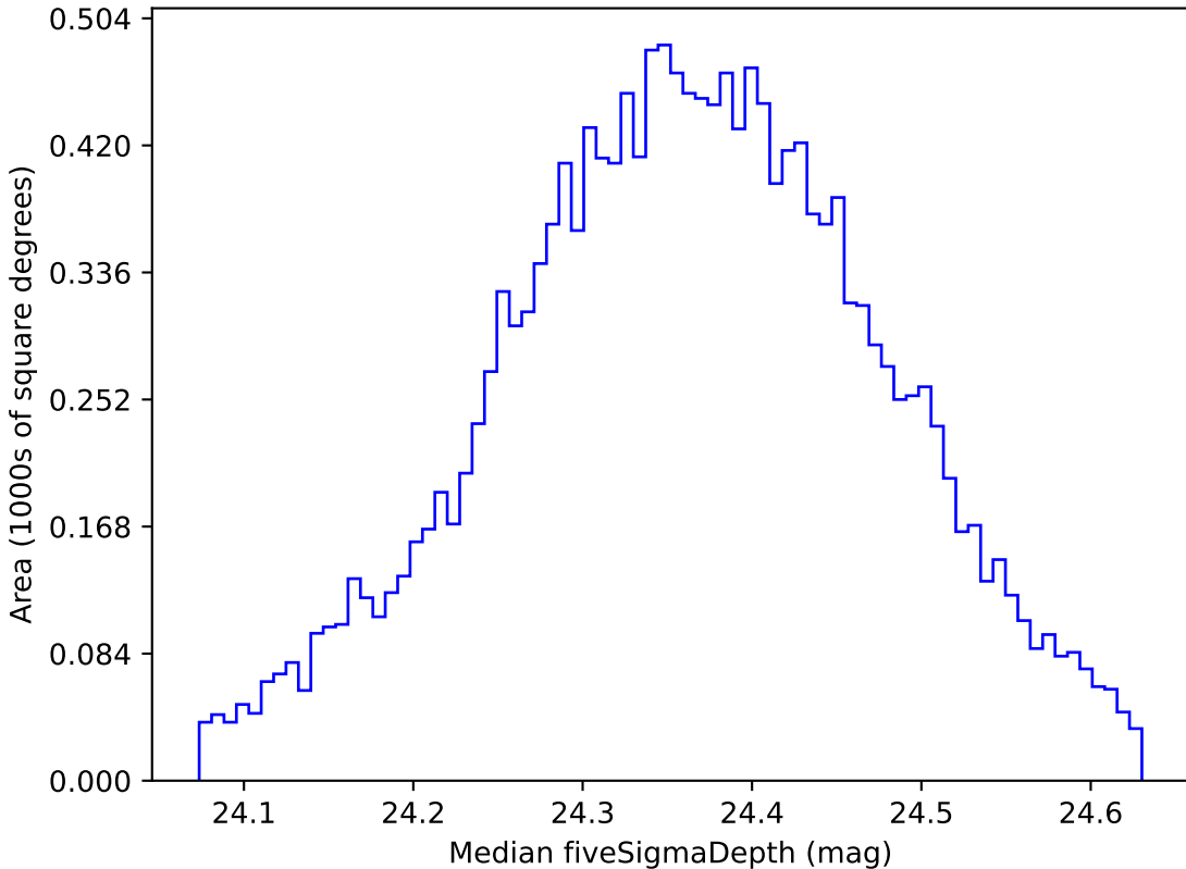
all_long_v3.4_10yrs WFD g band: Median fiveSigmaDepth
