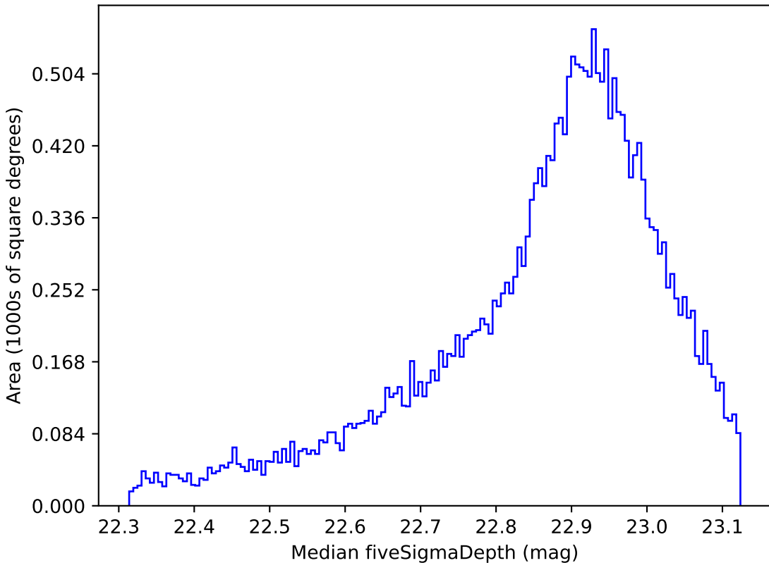
all_long_v3.4_10yrs All sky z band: Median fiveSigmaDepth
