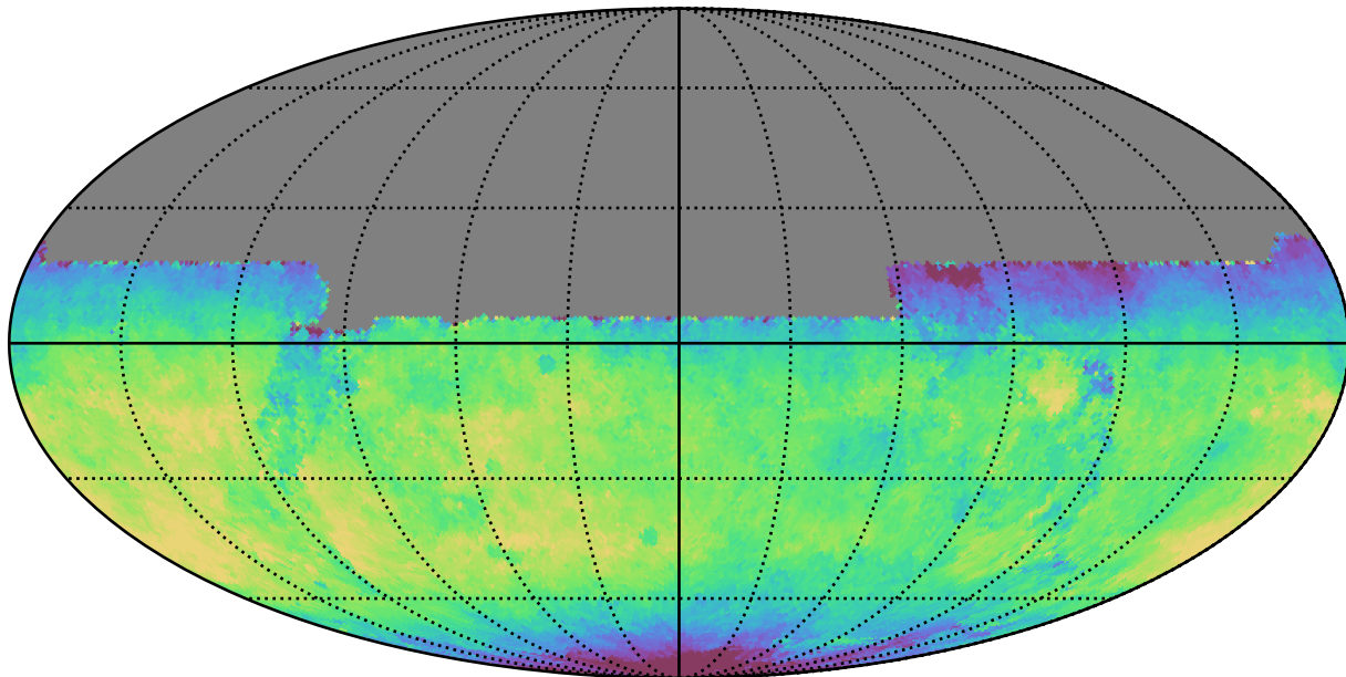
all_long_v3.4_10yrs All sky y band: Median fiveSigmaDepth
