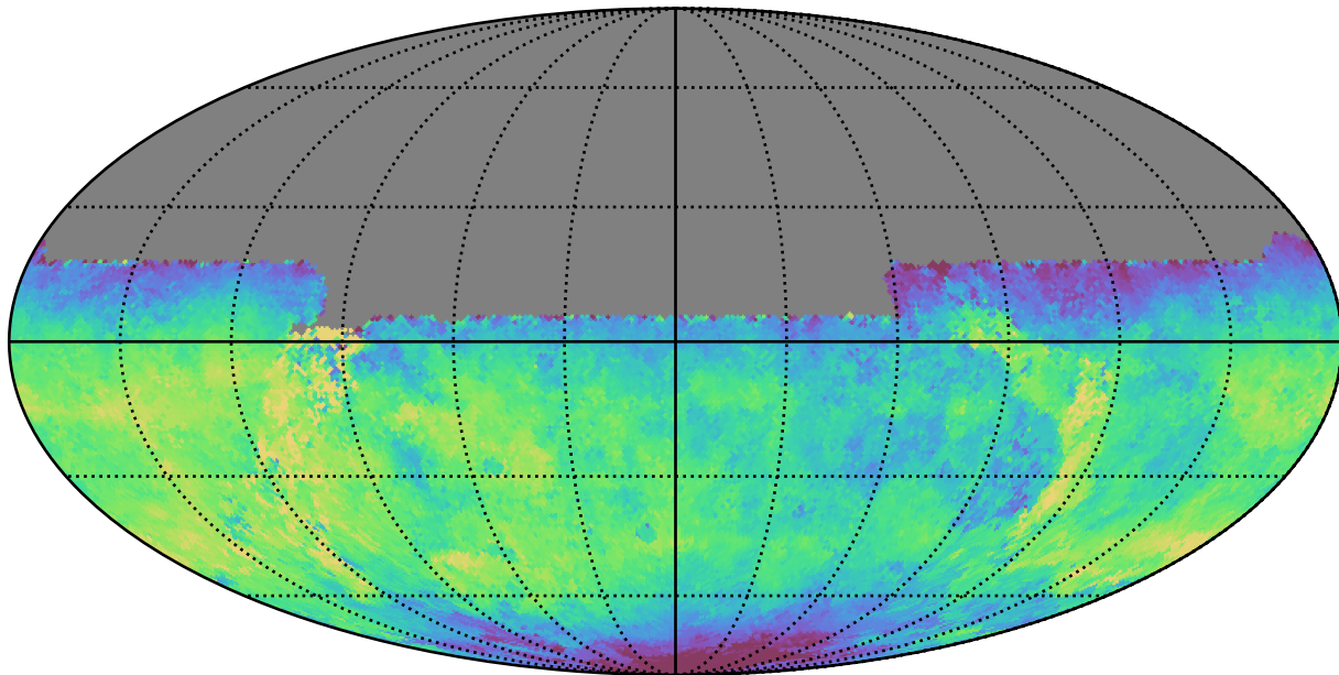
all_long_v3.4_10yrs All sky u band: Median fiveSigmaDepth
