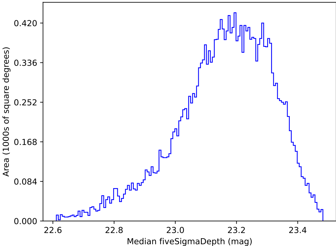
all_long_v3.4_10yrs All sky u band: Median fiveSigmaDepth
