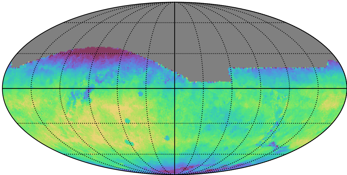
all_long_v3.4_10yrs All sky r band: Median fiveSigmaDepth
