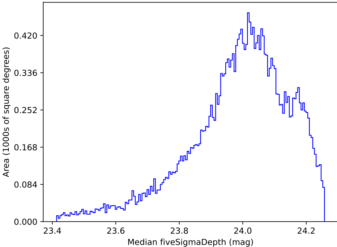
all_long_v3.4_10yrs All sky r band: Median fiveSigmaDepth
