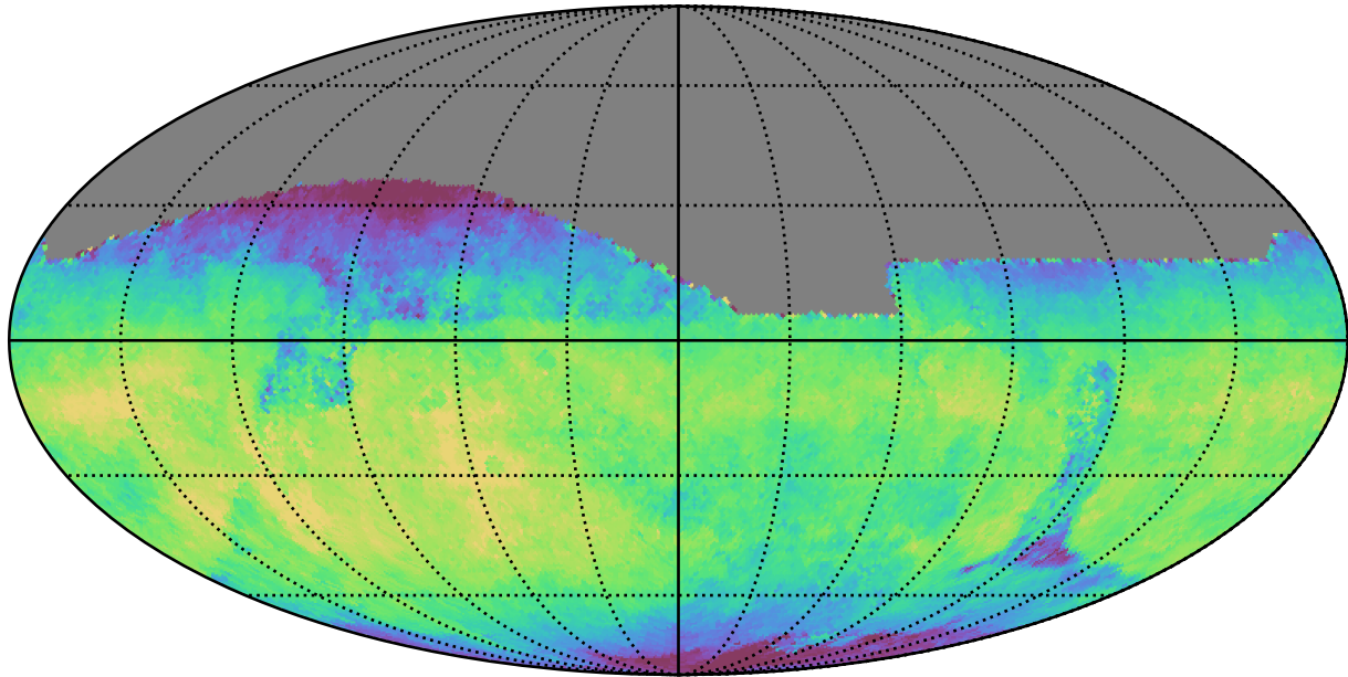
all_long_v3.4_10yrs All sky i band: Median fiveSigmaDepth
