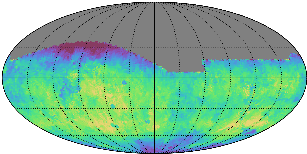
all_long_v3.4_10yrs All sky g band: Median fiveSigmaDepth
