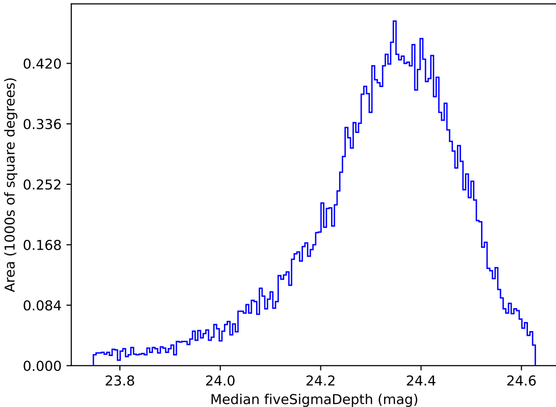
all_long_v3.4_10yrs All sky g band: Median fiveSigmaDepth
