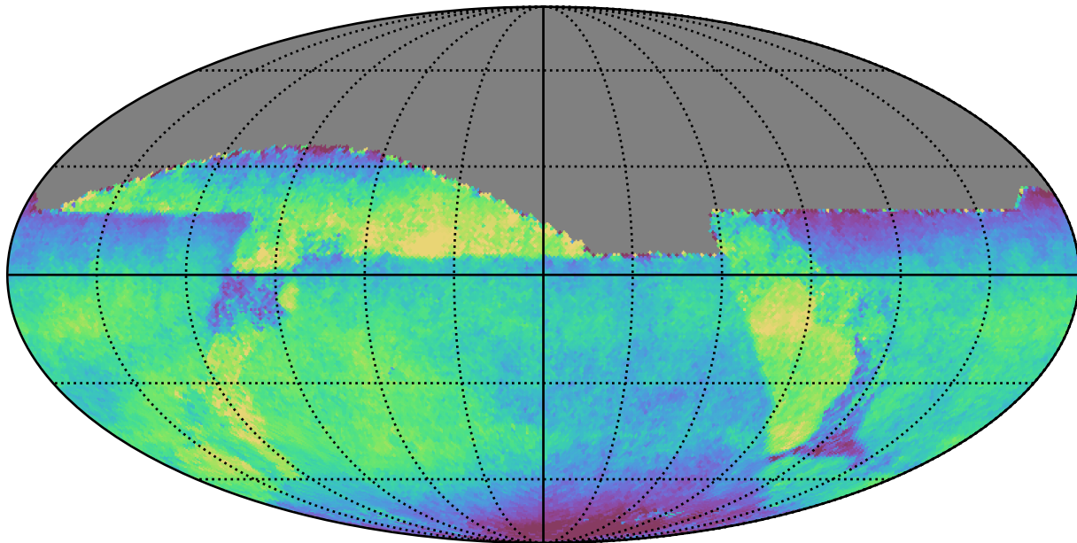
all_long_v3.4_10yrs All sky all bands: Median fiveSigmaDepth
