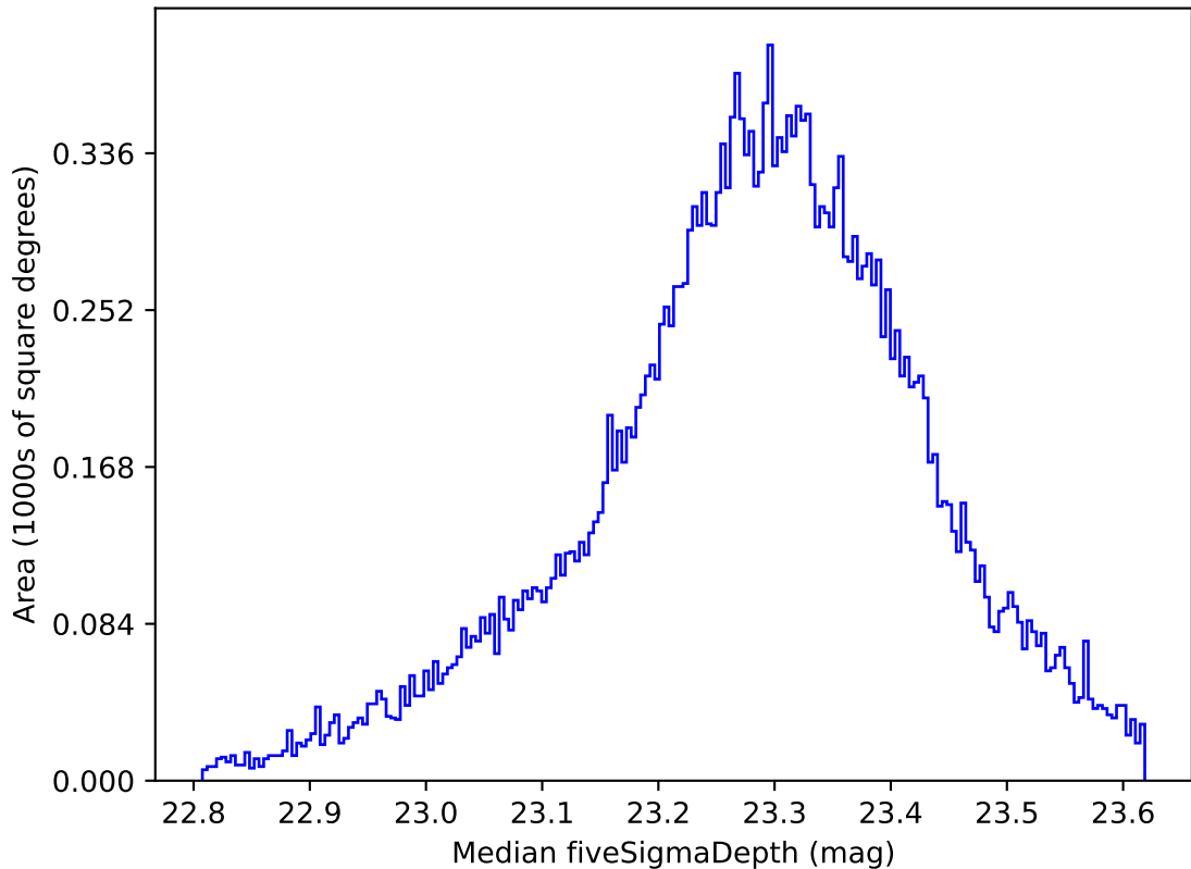
all_long_v3.4_10yrs All sky all bands: Median fiveSigmaDepth
