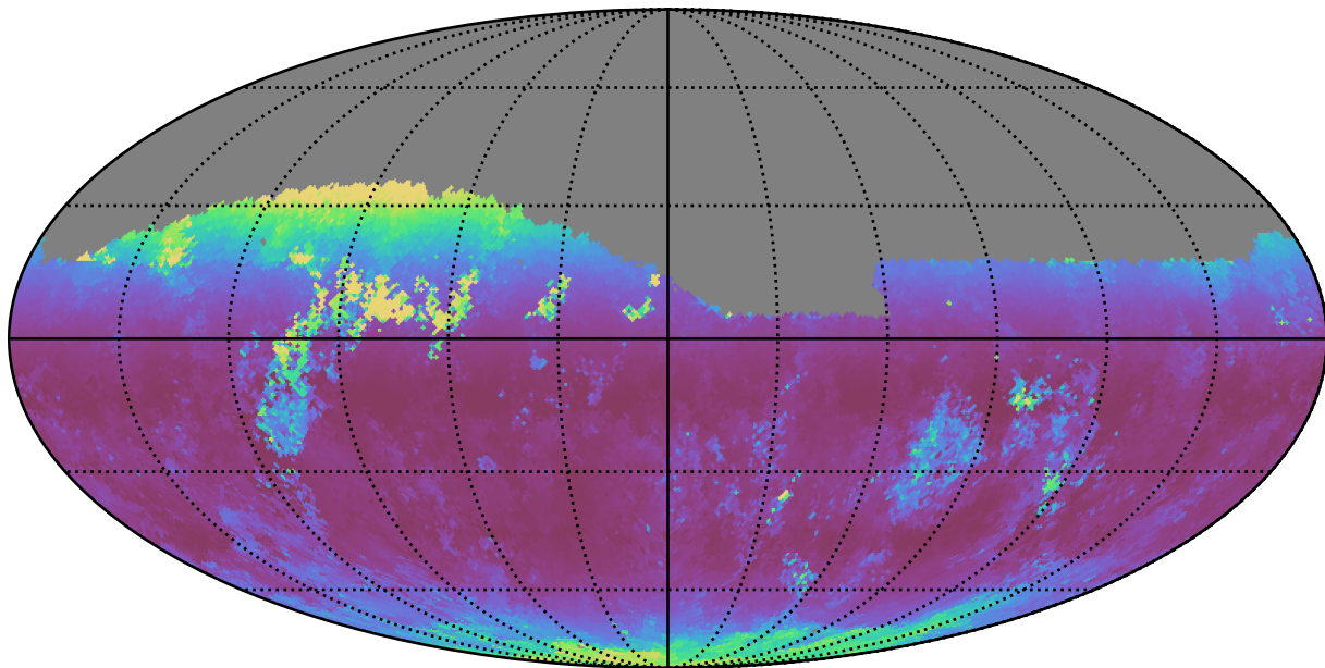
all_long_v3.4_10yrs Yr 1 z band: Median airmass
