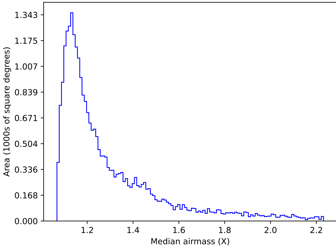
all_long_v3.4_10yrs Yr 1 z band: Median airmass
