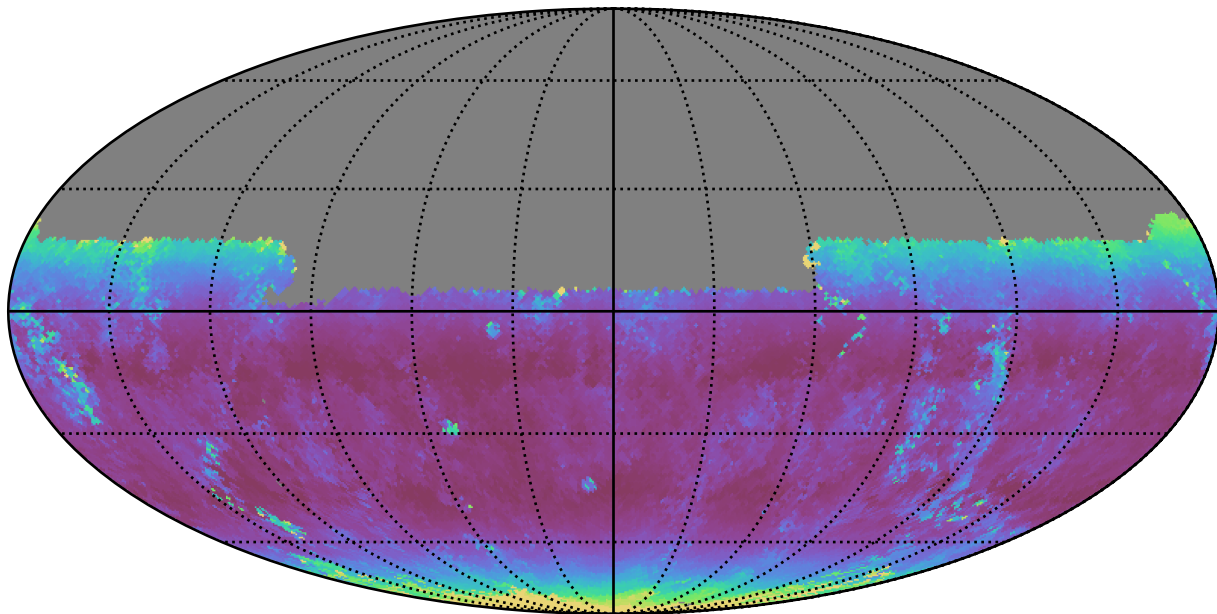
all_long_v3.4_10yrs Yr 1 y band: Median airmass
