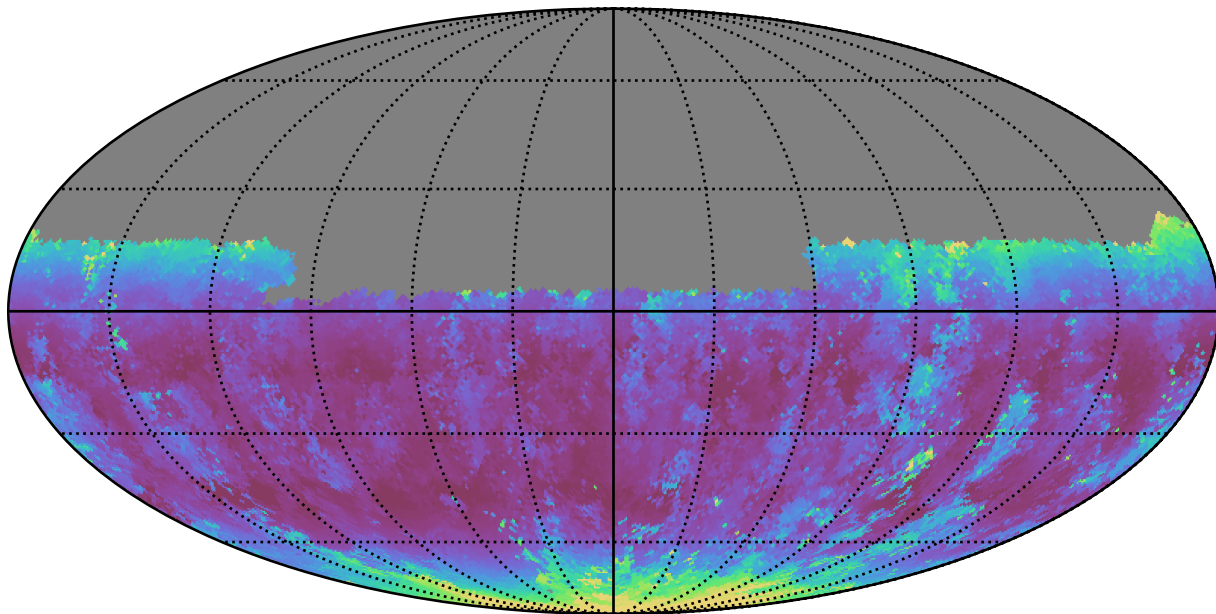
all_long_v3.4_10yrs Yr 1 u band: Median airmass
