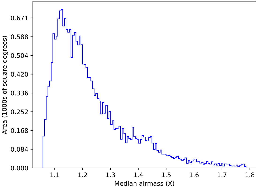
all_long_v3.4_10yrs Yr 1 u band: Median airmass
