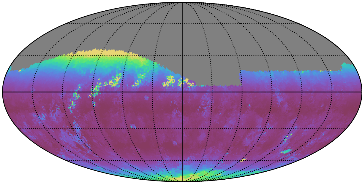
all_long_v3.4_10yrs Yr 1 r band: Median airmass
