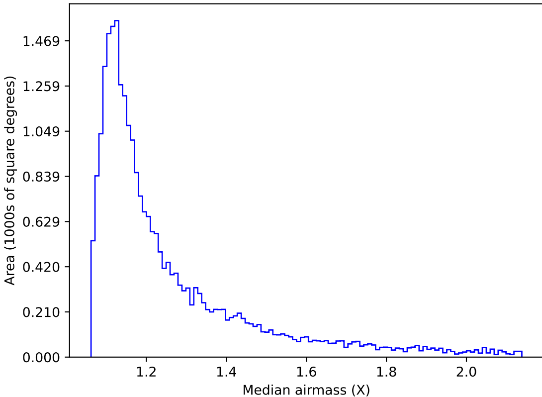
all_long_v3.4_10yrs Yr 1 r band: Median airmass
