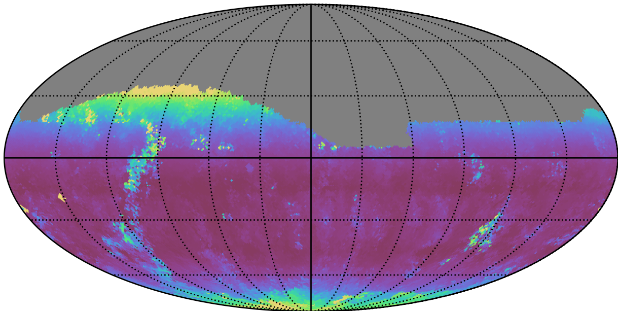
all_long_v3.4_10yrs Yr 1 i band: Median airmass
