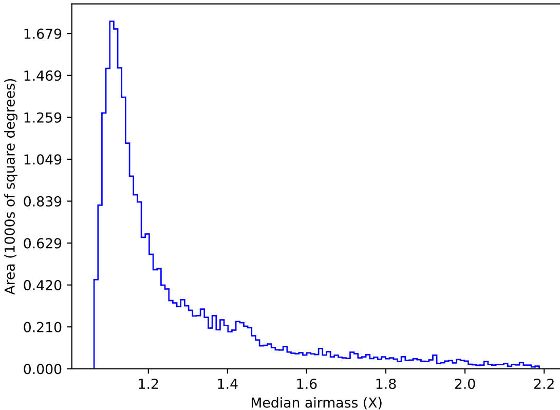
all_long_v3.4_10yrs Yr 1 i band: Median airmass
