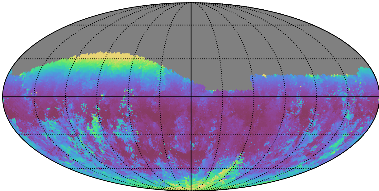
all_long_v3.4_10yrs Yr 1 g band: Median airmass
