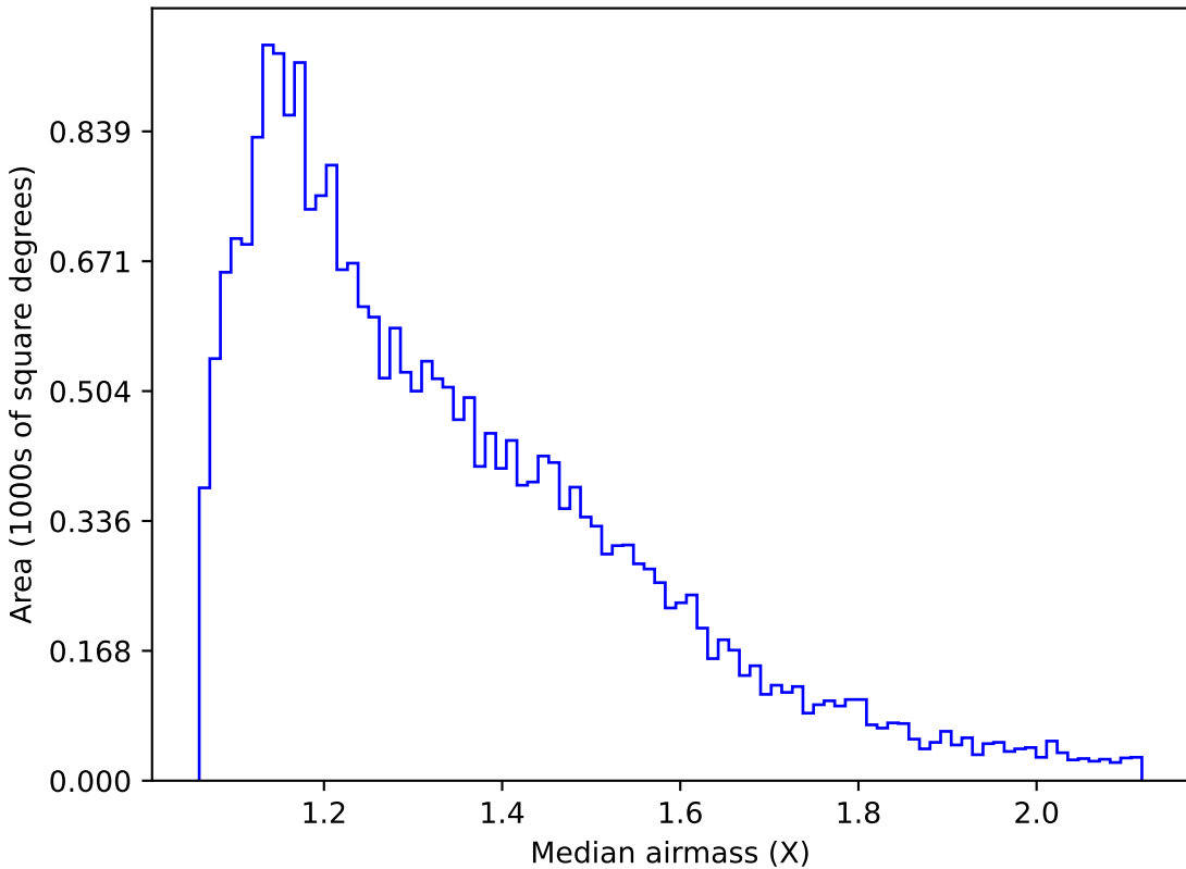
all_long_v3.4_10yrs Yr 1 g band: Median airmass
