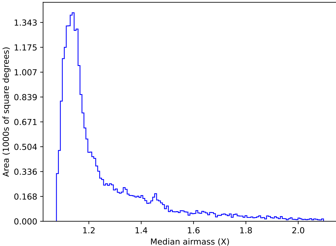
all_long_v3.4_10yrs Yr 1 all bands: Median airmass
