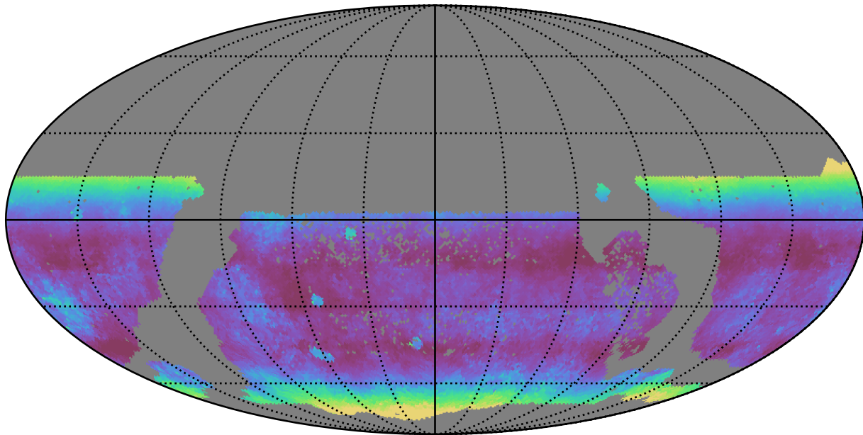
all_long_v3.4_10yrs WFD z band: Median airmass
