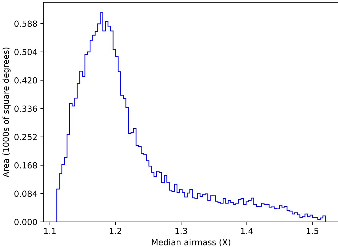
all_long_v3.4_10yrs WFD z band: Median airmass
