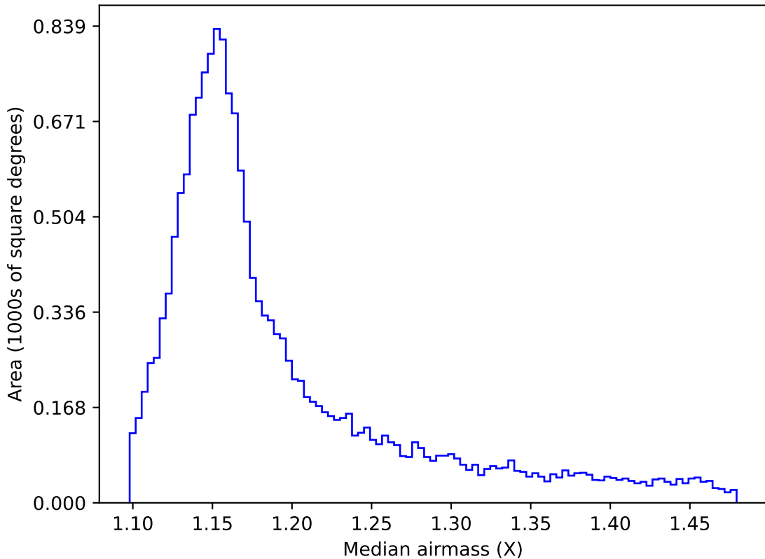
all_long_v3.4_10yrs WFD y band: Median airmass
