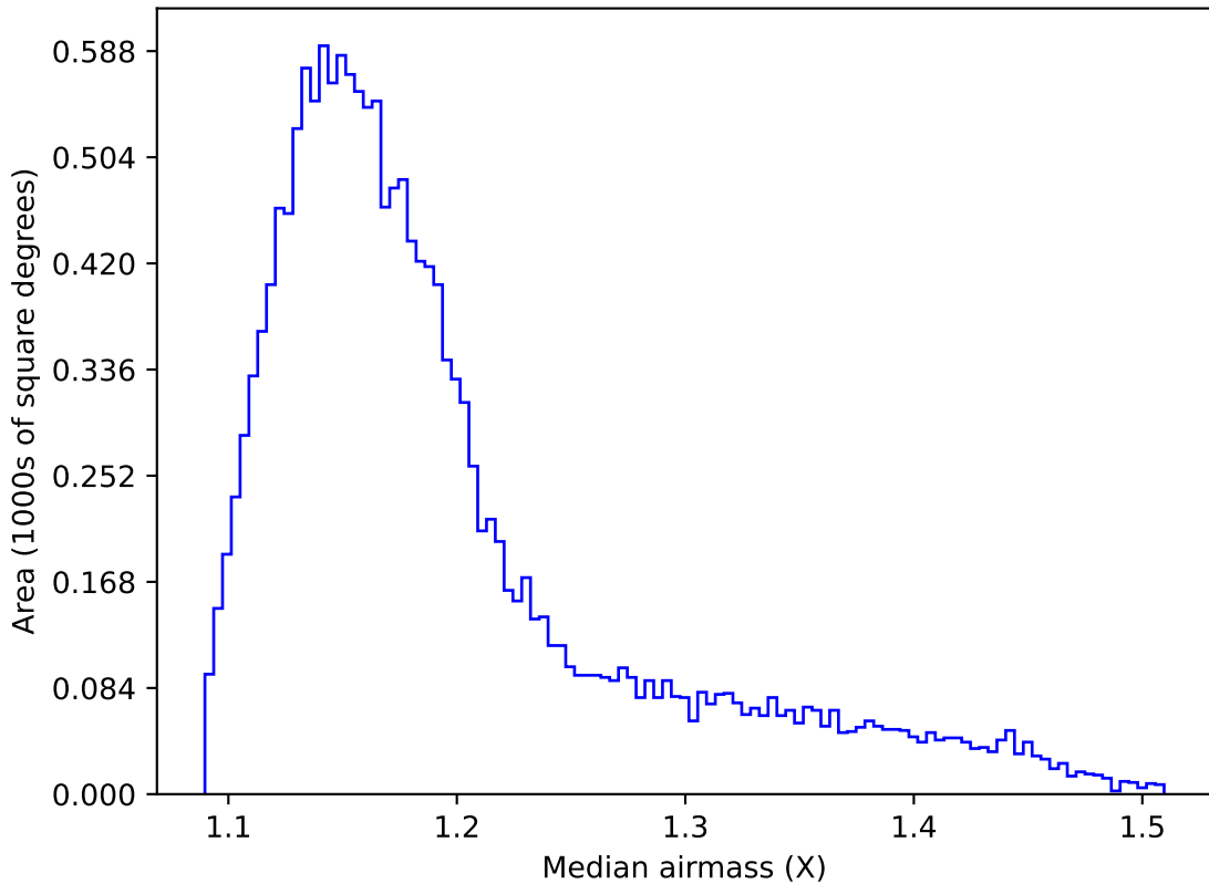
all_long_v3.4_10yrs WFD r band: Median airmass
