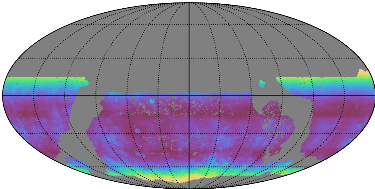
all_long_v3.4_10yrs WFD i band: Median airmass
