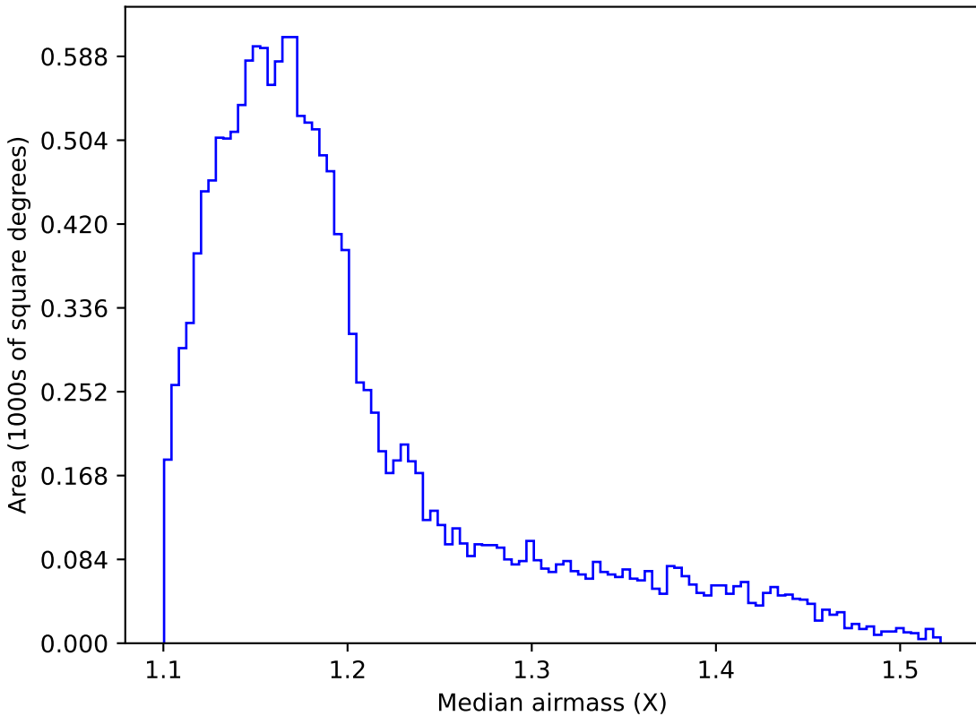
all_long_v3.4_10yrs WFD i band: Median airmass
