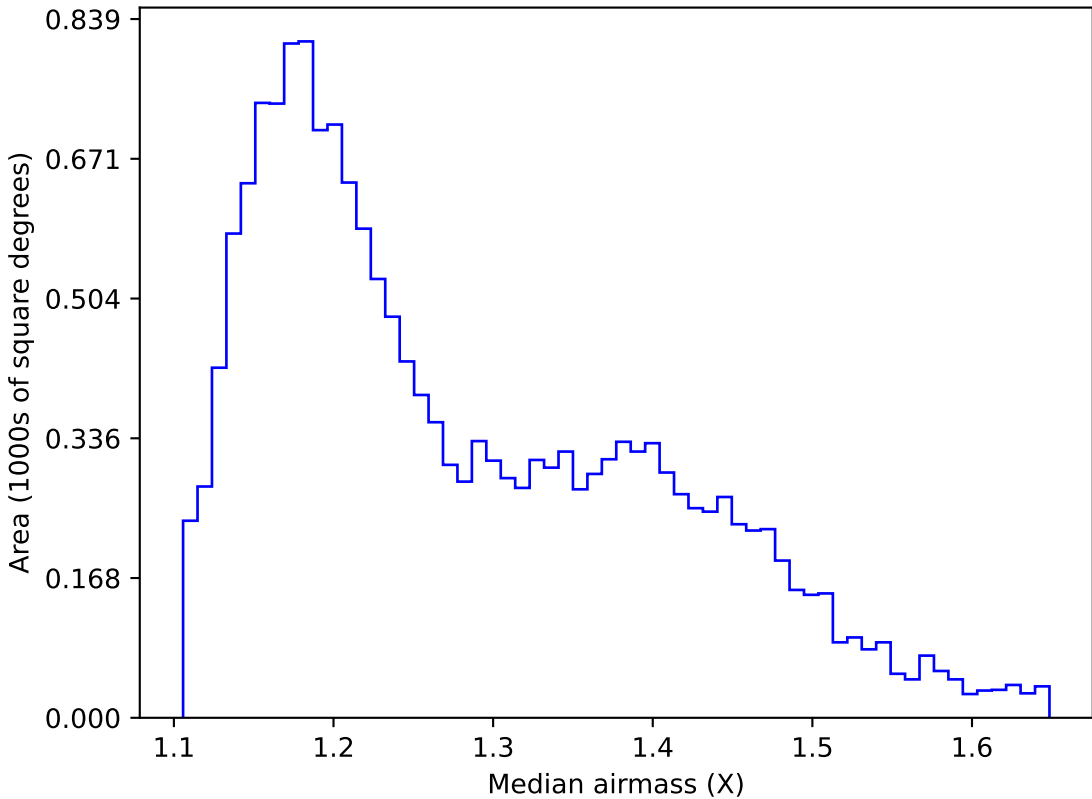
all_long_v3.4_10yrs WFD g band: Median airmass
