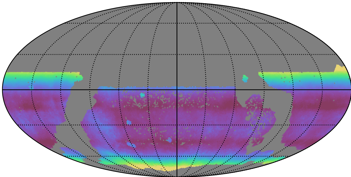
all_long_v3.4_10yrs WFD all bands: Median airmass
