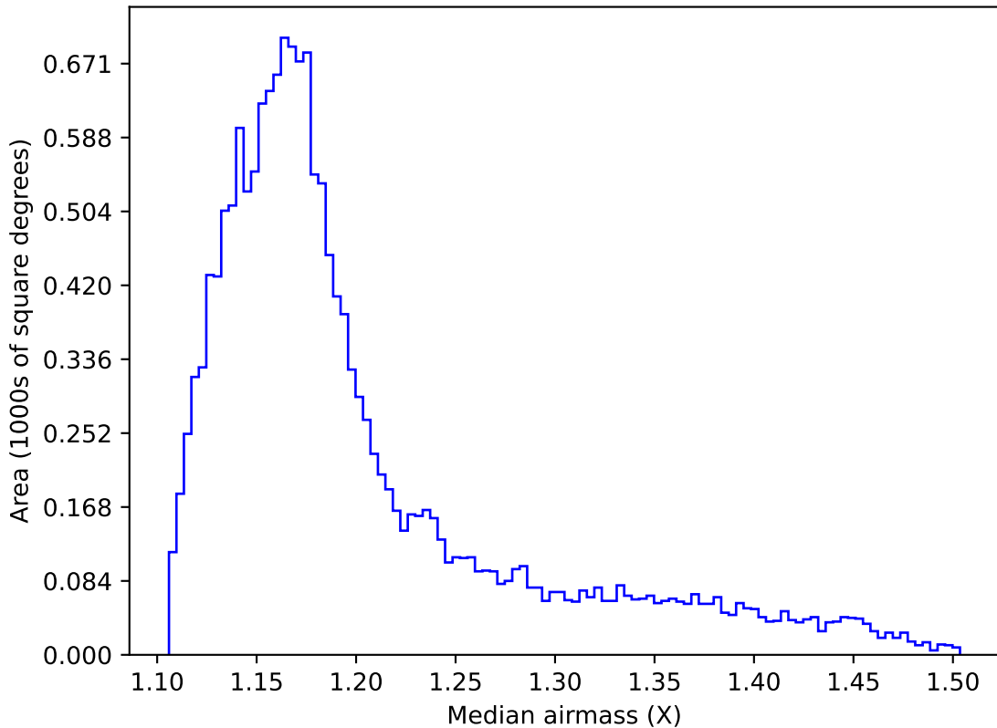
all_long_v3.4_10yrs WFD all bands: Median airmass
