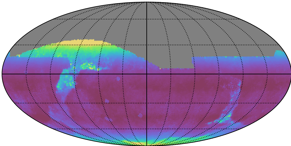
all_long_v3.4_10yrs All sky z band: Median airmass
