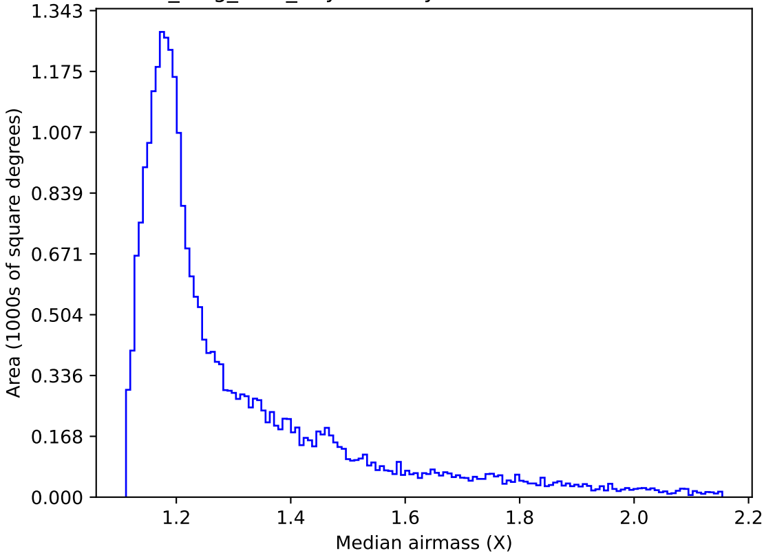
all_long_v3.4_10yrs All sky z band: Median airmass
