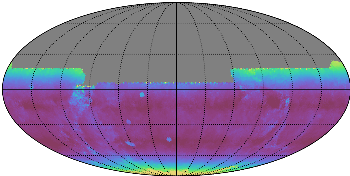
all_long_v3.4_10yrs All sky y band: Median airmass
