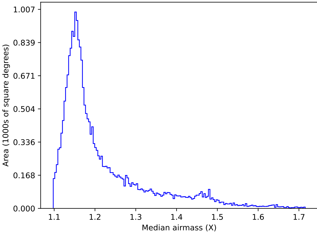
all_long_v3.4_10yrs All sky y band: Median airmass
