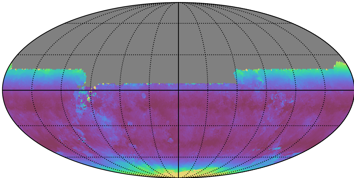
all_long_v3.4_10yrs All sky u band: Median airmass
