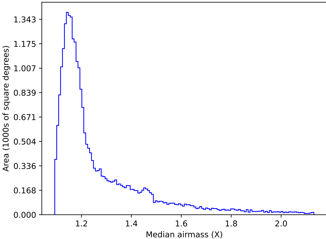
all_long_v3.4_10yrs All sky r band: Median airmass
