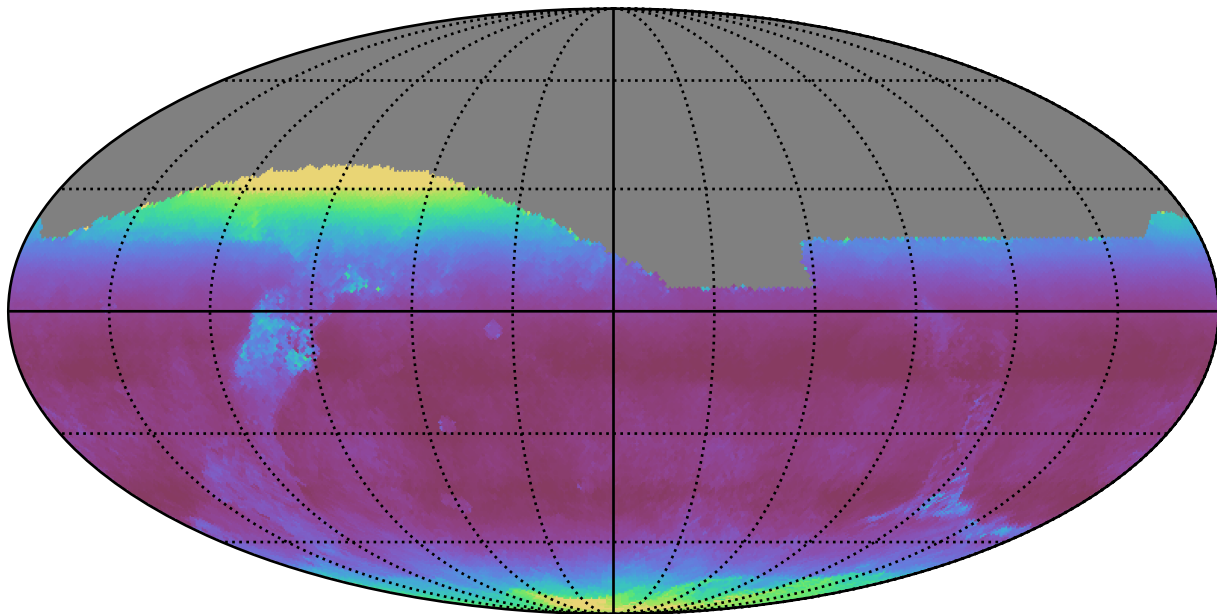
all_long_v3.4_10yrs All sky i band: Median airmass
